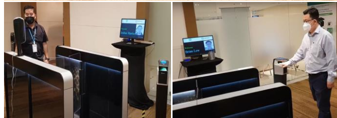
IDEMIA MorphoWave XP & VisionPass integrated with elegant sensor barrier Argus 80 from Dormakaba
